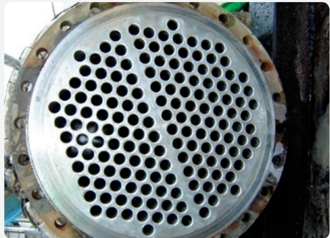
AFTER CLEANING
