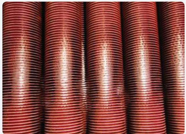
BEFORE & AFTER AIR FIN FAN COOLER CHEMICAL CLEANING
