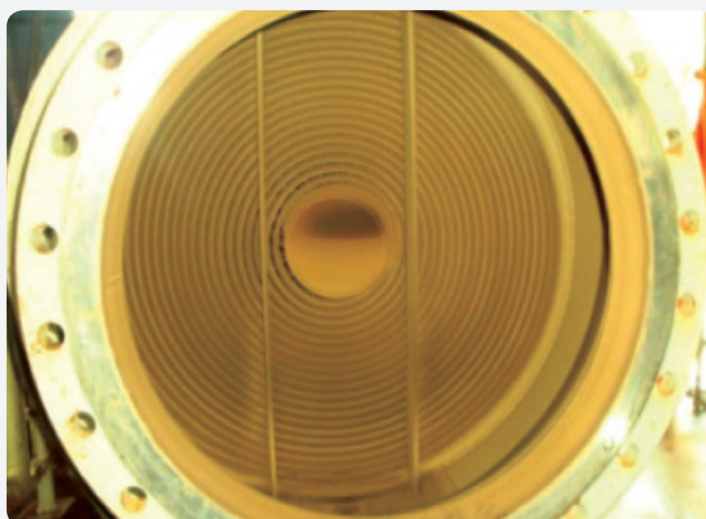
BEFORE CLEANING
