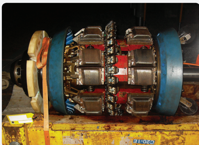
INTELLIGENT PIGGING
